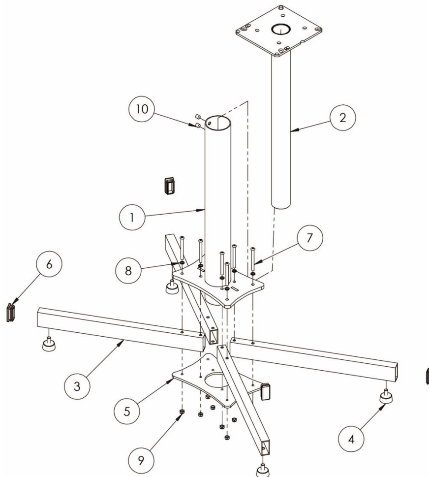
Floor Stand 3 Assembly Drawing
